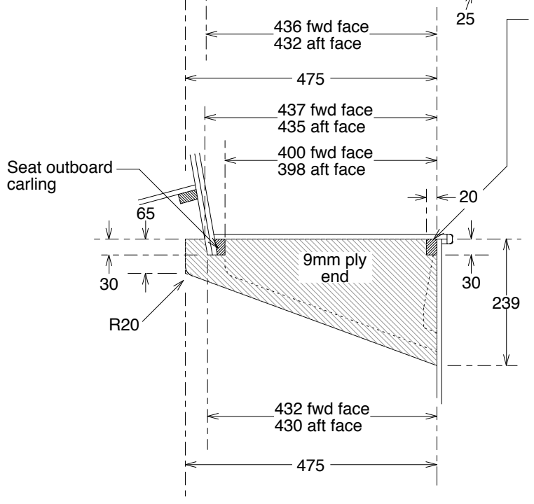
Aft Gutter Assembly
