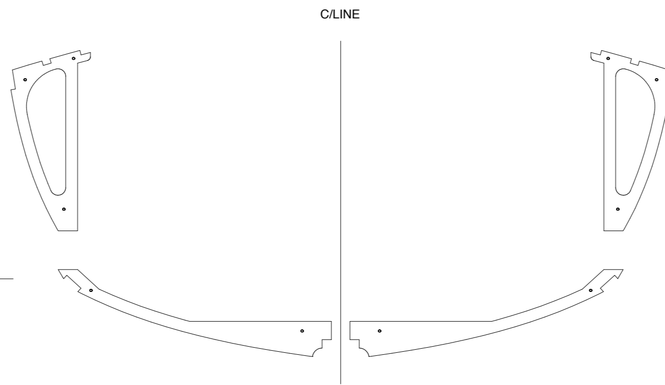
FRAME -2250 MID LAYER 6MM PLY
