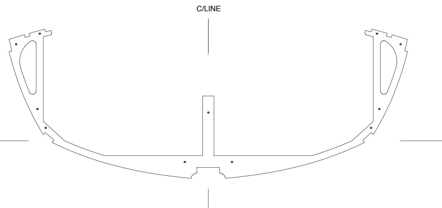
FRAME -3200 AFT LAYER 6MM PLY
