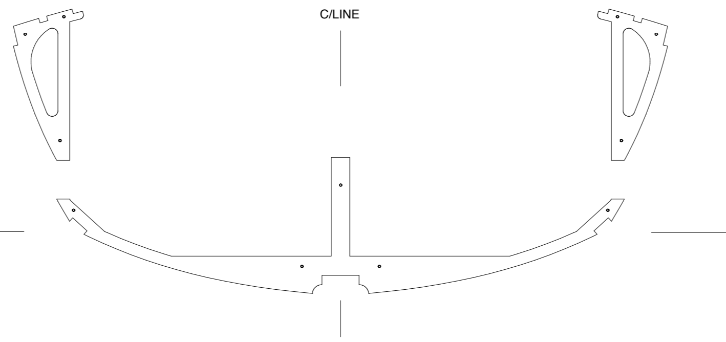
FRAME -3200 MID LAYER 6MM PLY
