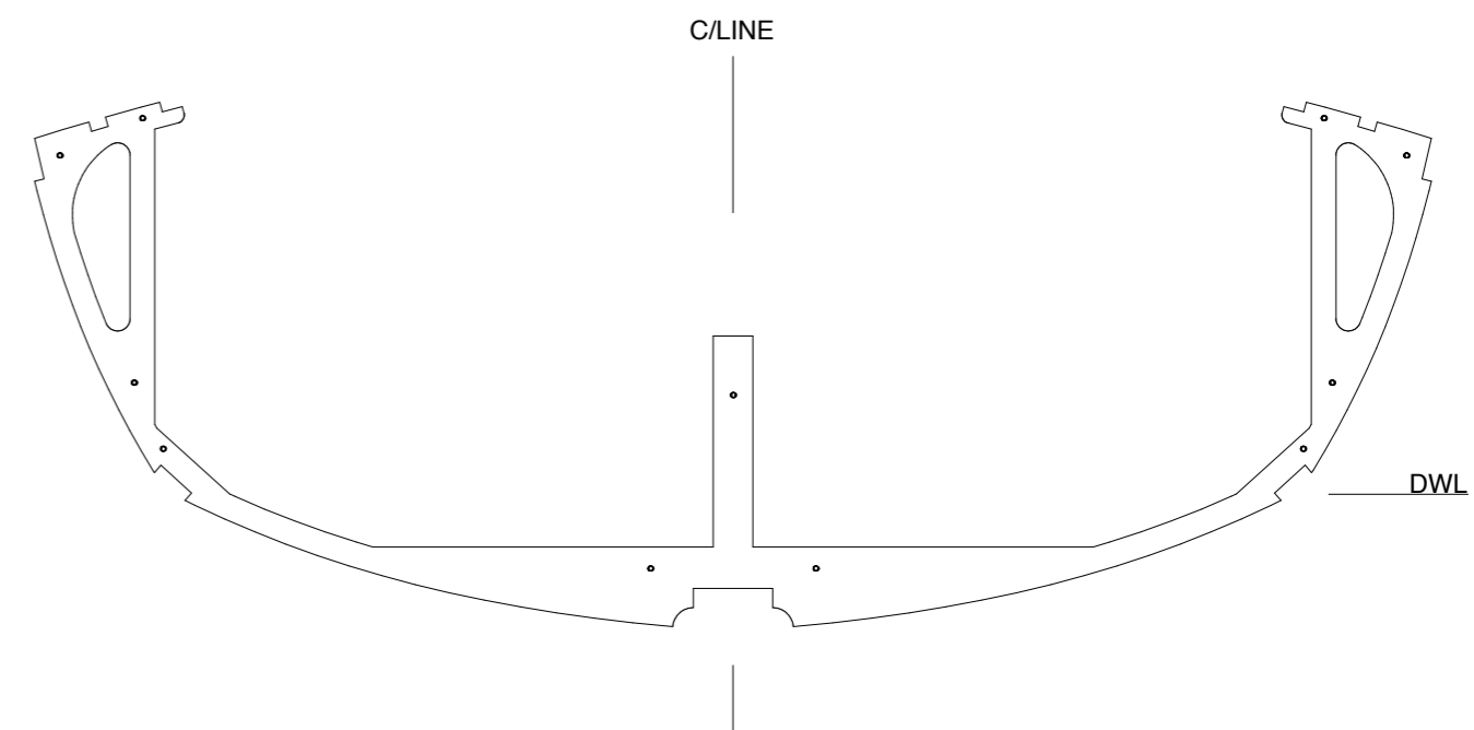
FRAME -3200 FWD LAYER 6MM PLY
