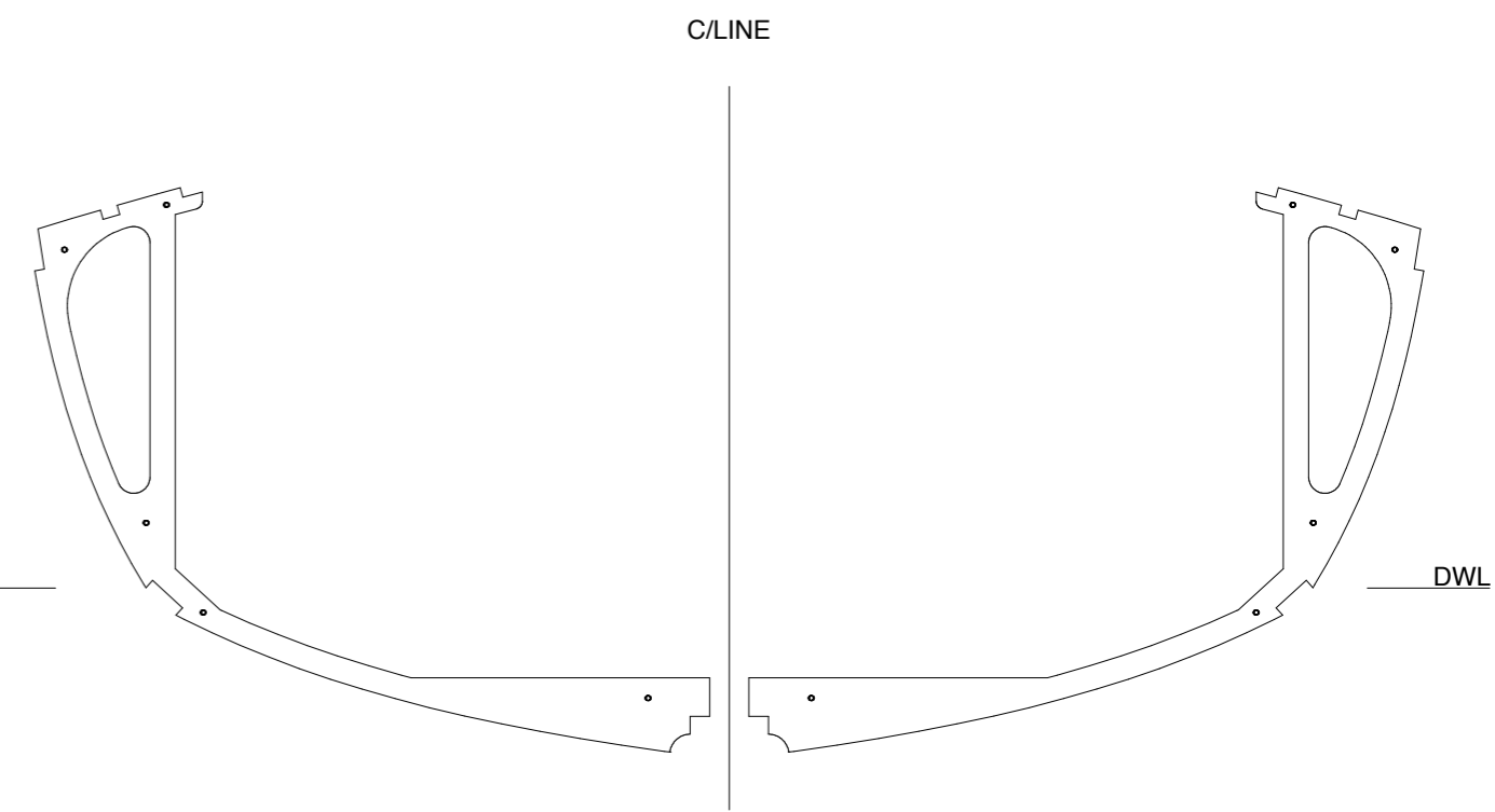
FRAME -2250 FWD LAYER 6MM PLY
