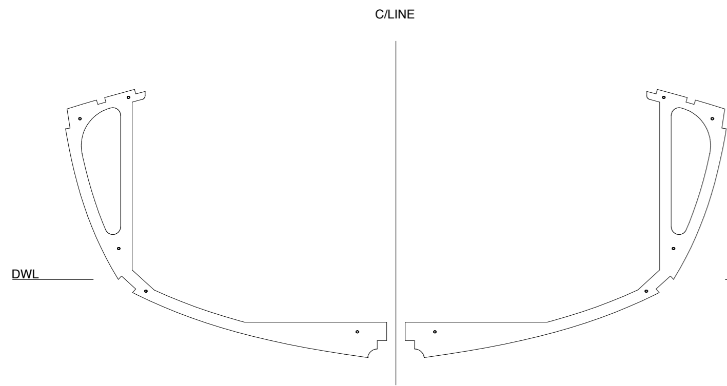
FRAME -2250 AFT LAYER 6MM PLY
